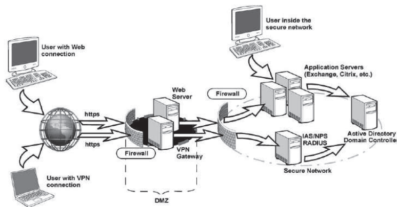
Figura 3.29: Firewall e DMZ
