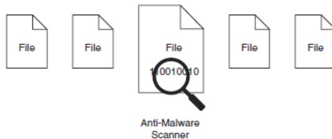
Figura 3.28: File Scanning
